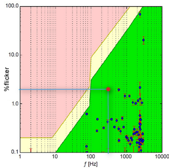
Figure 4 – %flicker vs. Flicker frequency
