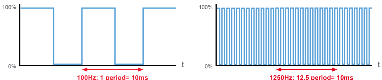
Figure 3 – Frequency
